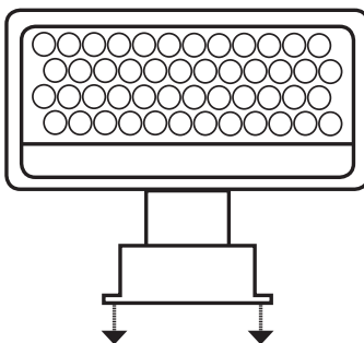
SPLASHLIGHT™ Wall Washer 3/8" mounting holes
